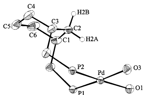
Figure 2. A plot showing the chair conformation of the cyclohexane skeleton in 6 including the hydrogens on C2; bond angles (deg) with estimated standard deviations: C1–C2–C3 115.2 (3), C2–C3–C4 109.0(3), C3–C4–C5 113.3(3), C4–C5–C6 112.2(4), C5–C6–C1 = 112.9(3), C6–C1–C2 108.8 (3)
