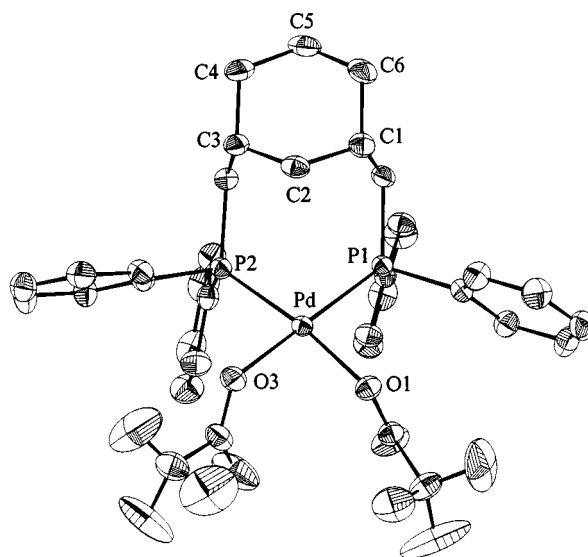
Figure 1. Perspective view (DIAMOND) of 6 (thermal ellipsoids at 30% probability); bond lengths (Å) and angles (deg) with estimated standard deviations: Pd–O1 2.086(2), Pd–O3 2.074(2), Pd–P1 2.261(1), Pd–P2 2.252(1), O1–Pd–O3 83.36(10), P1–Pd–P2 93.81(4), P1–Pd–O1 93.36(8), P1–Pd–O3 173.83(7)
